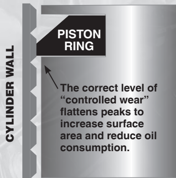
Fig. 2: Broken-In Cylinder
